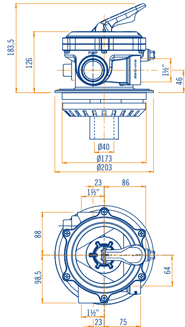
Válvula selectora Top Flat 1 1/2" 1 1/2" Top Flat selector valve
