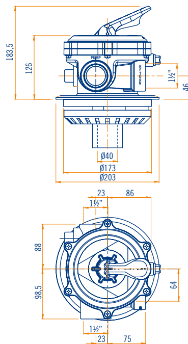
Vanne multivoies Top Flat 1 1/2" 1 1/2" Top Flat selector valve
