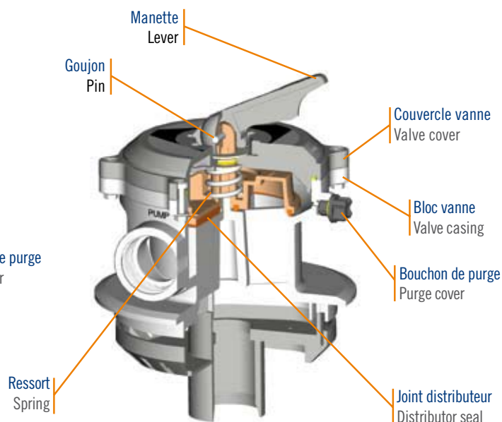
Vanne multivoies Top Flat 1 1/2" 1 1/2" Top Flat selector valve
