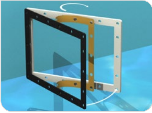
Figure 52 – Apposez le second joint
